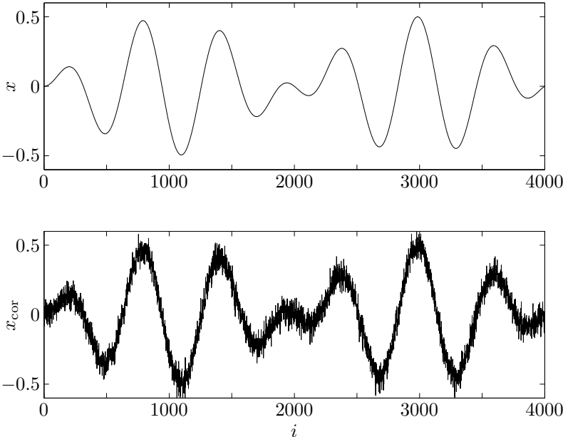
Figure 6.8 Top: the original signal x \in \mathbf{R}^{4000} . Bottom: the corrupted signal x_{cor} .
