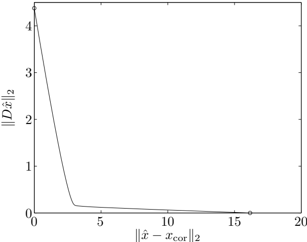
Figure 6.9 Optimal trade-off curve between \|D\hat{x}\|_2 and \|\hat{x} - x_{cor}\|_2 . The curve has a clear knee near \|\hat{x} - x_{cor}\|_2 \approx 3 .
